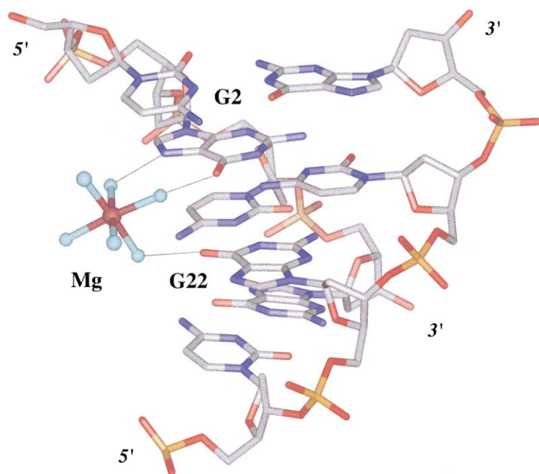
Figure 1. Coordination of \text{Mg}^{2+} at the CpG Step Near One End of the DDD [3]
