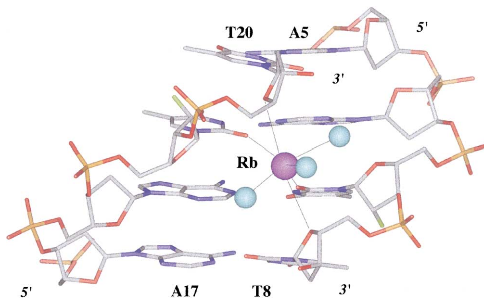
Figure 3. Coordination of \text{Rb}^+ at the Central ApT Step in the DDD [26]
