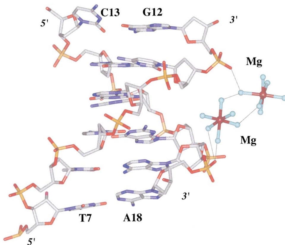
Figure 2. Bridging of Phosphate Groups by Two \text{Mg}^{2+} across the Minor Groove of the DDD [29]
